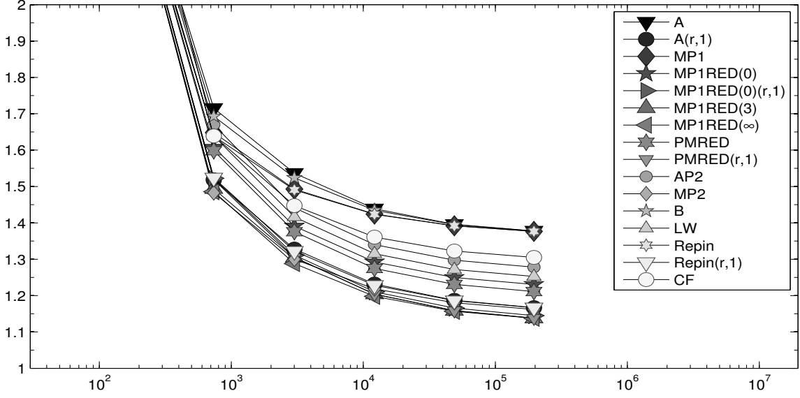
FIGURE 7.6. History of efficiency indices \eta_{xyz}/\|e\|_{\text{NC}} of various a posteriori error estimators \eta_{xyz} labelled xyz in the figure as functions of the number of unknowns on uniform meshes in Subsection 7.3.
