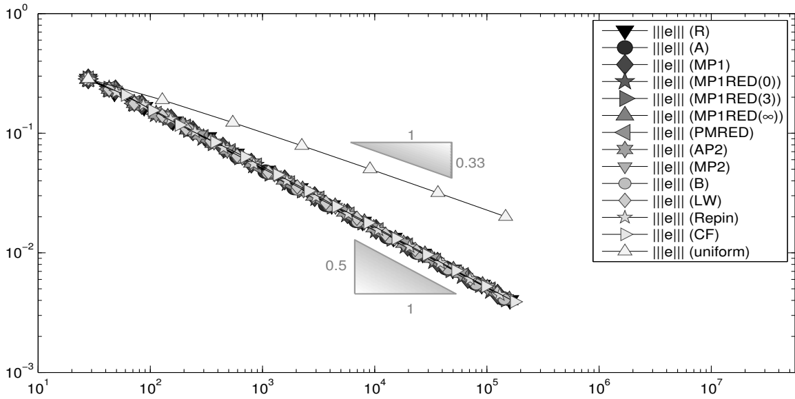
FIGURE 7.3. Convergence history of the energy error for uniform and adaptive mesh-refinements in Subsection 7.1.
