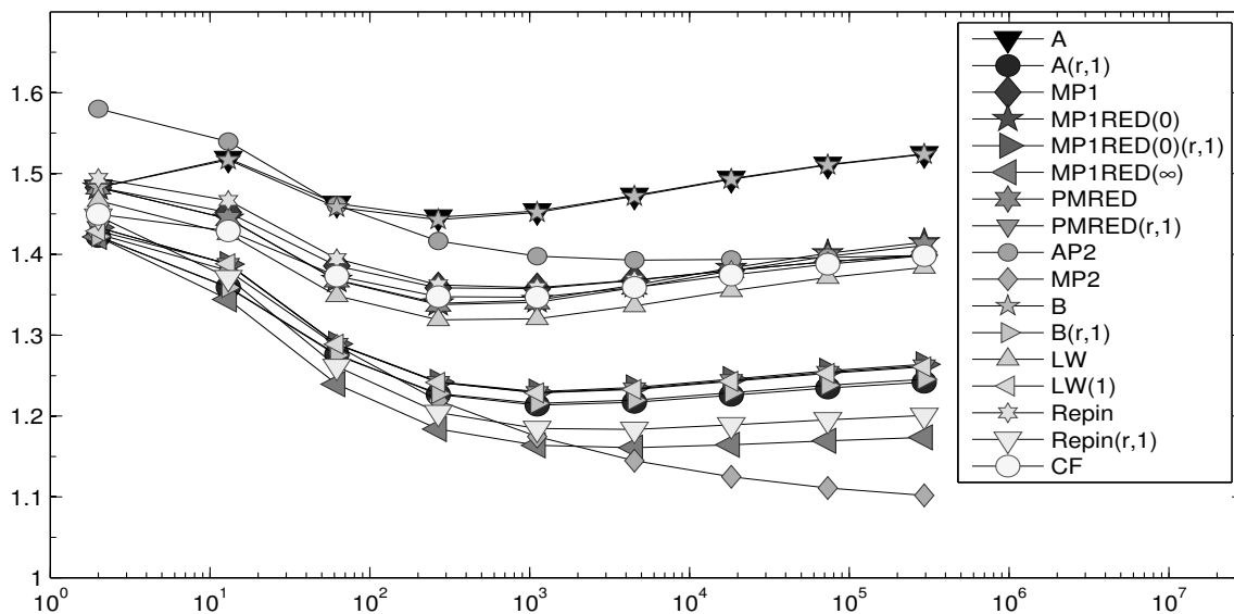
FIGURE 7.9. History of efficiency indices \eta_{xyz}/\|e\|_{\text{NC}} of various a posteriori error estimators \eta_{xyz} labelled xyz in the figure as functions of the number of unknowns on uniform meshes in Subsection 7.4.
