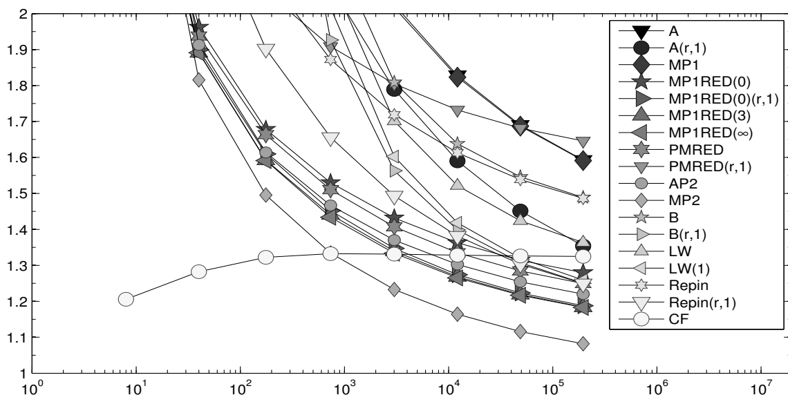
FIGURE 7.15. History of efficiency indices \eta_{xyz}/\|e\|_{NC} of various a posteriori error estimators \eta_{xyz} labelled xyz in the figure as functions of the number of unknowns on uniform meshes in Subsection 7.6.
