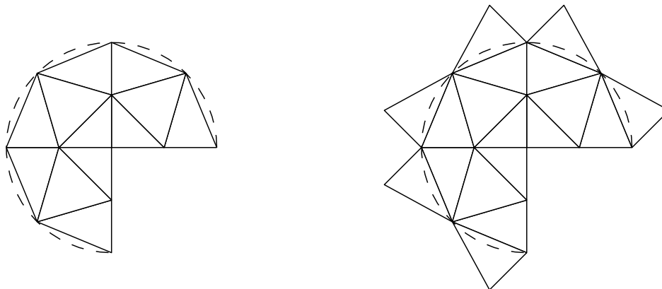
FIGURE 7.8. Triangulation \mathcal{T} (left, solid lines) and extended triangulation \hat{\mathcal{T}} (right, solid lines) with \bigcup \mathcal{T} \subseteq \Omega \subseteq \bigcup \hat{\mathcal{T}} for the sector domain \Omega (dashed lines) from Section 7.4.
