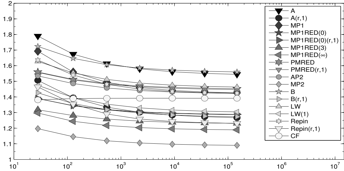
FIGURE 7.1. History of efficiency indices \eta_{xyz}/\|e\|_{NC} of various a posteriori error estimators \eta_{xyz} labelled xyz in the figure as functions of the number of unknowns on uniform meshes in Subsection 7.1.
