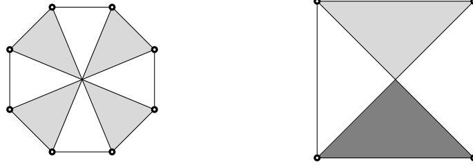
FIGURE 7.11. Distribution of \kappa = 1 (white) and \kappa = 1000 (lightgray) in octagon domain of Subsection 7.6 (left) and distribution of \kappa = 1 (white), \kappa = 100 (lightgray) and \kappa = 10000 (darkgray) in square domain of Subsection 7.5.
