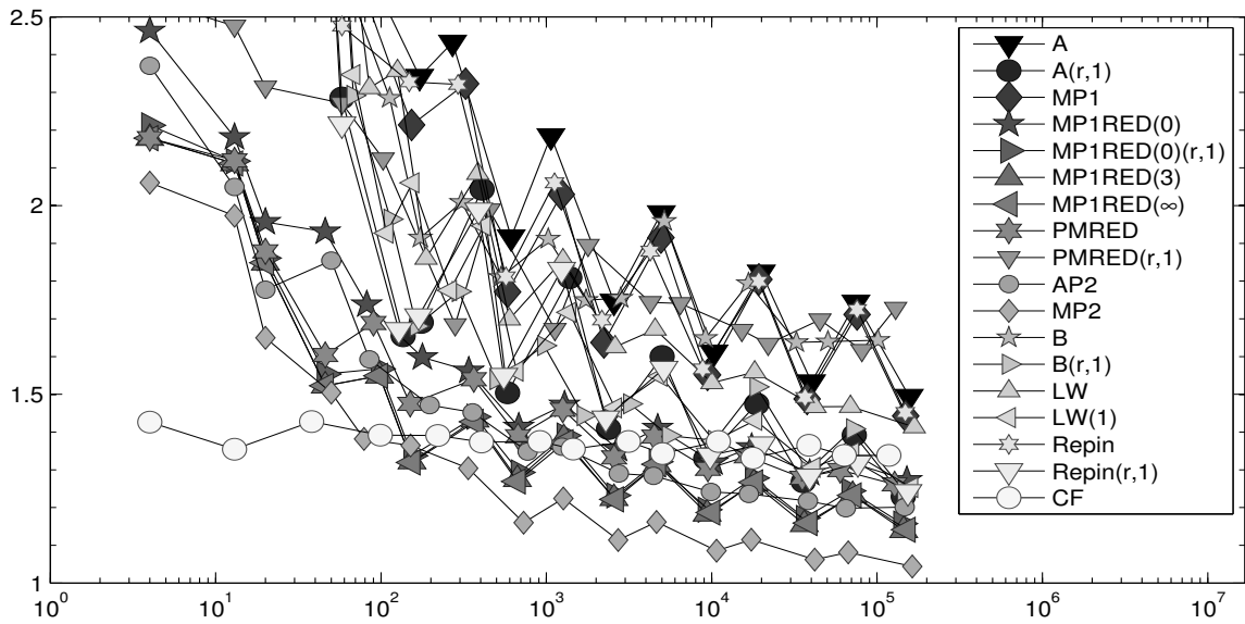
FIGURE 7.13. History of efficiency indices \eta_{xyz}/|||e|||_{NC} of various a posteriori error estimators \eta_{xyz} labelled xyz in the figure as functions of the number of unknowns on adaptive meshes in Subsection 7.5.
