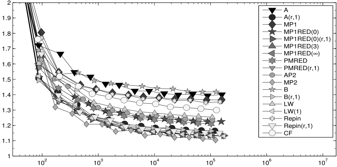
FIGURE 7.7. History of efficiency indices \eta_{xyz}/\|e\|_{\text{NC}} of various a posteriori error estimators \eta_{xyz} labelled xyz in the figure as functions of the number of unknowns on adaptive meshes in Subsection 7.3.
