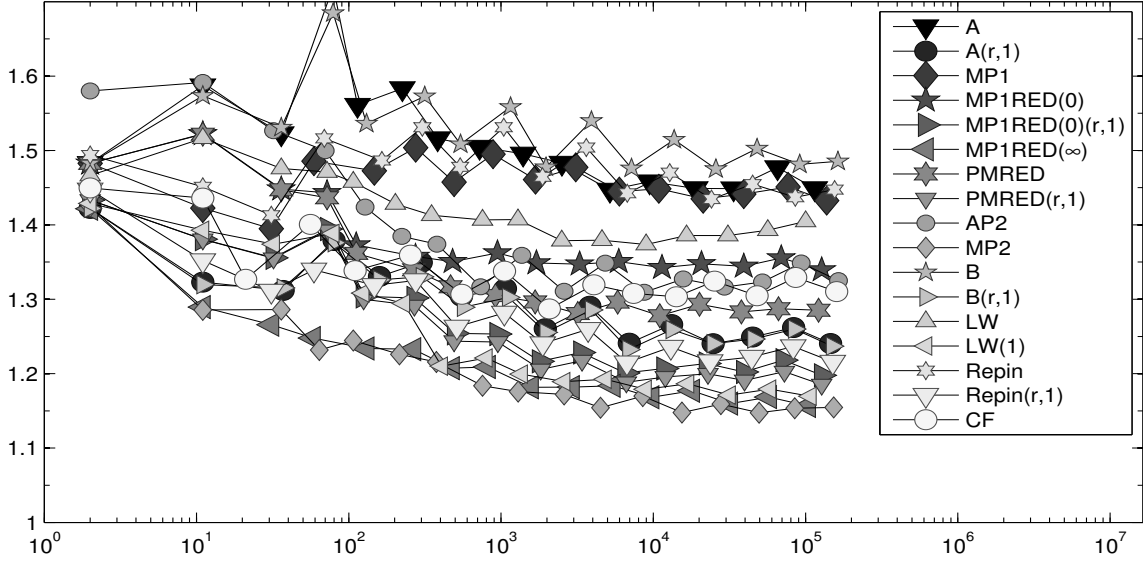
FIGURE 7.10. History of efficiency indices \eta_{xyz}/|||e|||_{NC} of various a posteriori error estimators \eta_{xyz} labelled xyz in the figure as functions of the number of unknowns on adaptive meshes in Subsection 7.4.
