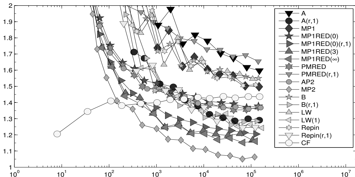
FIGURE 7.16. History of efficiency indices \eta_{xyz}/\|e\|_{\text{NC}} of various a posteriori error estimators \eta_{xyz} labelled xyz in the figure as functions of the number of unknowns on adaptive meshes in Subsection 7.6.
