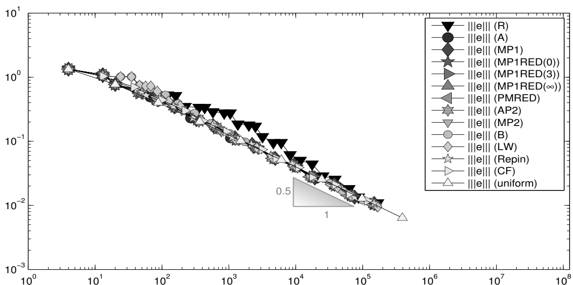
FIGURE 7.14. Convergence history of the energy error for uniform and adaptive mesh-refinements in Subsection 7.5.
