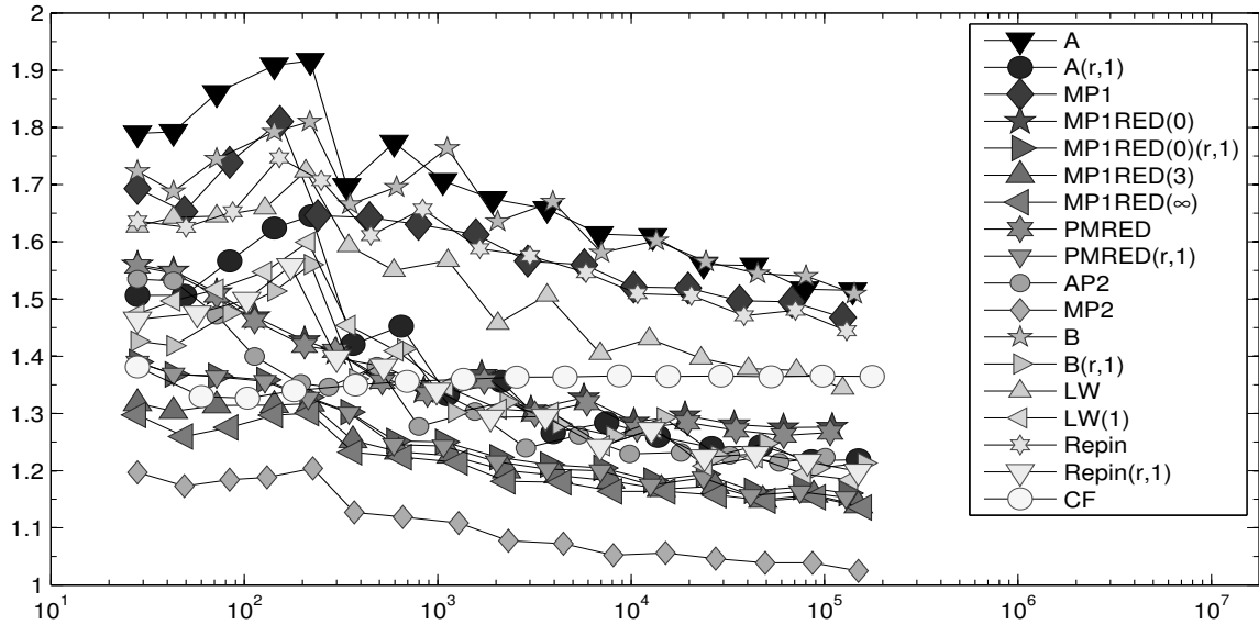
FIGURE 7.2. History of efficiency indices \eta_{xyz}/\|e\|_{NC} of various a posteriori error estimators \eta_{xyz} labelled xyz in the figure as functions of the number of unknowns on adaptive meshes in Subsection 7.1.
