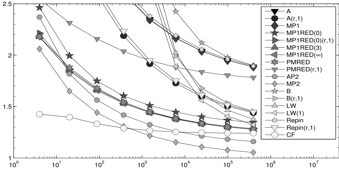
FIGURE 7.12. History of efficiency indices \eta_{xyz}/|||e|||_{NC} of various a posteriori error estimators \eta_{xyz} labelled xyz in the figure as functions of the number of unknowns on uniform meshes in Subsection 7.5.
