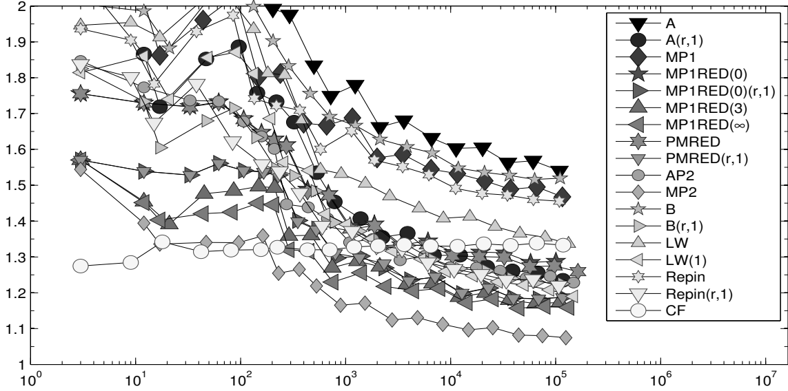
FIGURE 7.5. History of efficiency indices \eta_{xyz}/\|e\|_{\text{NC}} of various a posteriori error estimators \eta_{xyz} labelled xyz in the figure as functions of the number of unknowns on adaptive meshes in Subsection 7.2.
