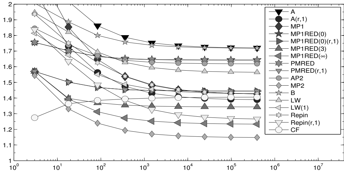
FIGURE 7.4. History of efficiency indices \eta_{xyz}/\|e\|_{NC} of various a posteriori error estimators \eta_{xyz} labelled xyz in the figure as functions of the number of unknowns on uniform meshes in Subsection 7.2.
