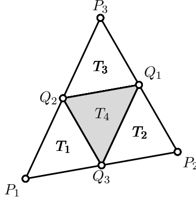
FIGURE 4.2. Central subtriangle T_4 = \text{conv}\{\text{mid}(\mathcal{E}(T))\} in \text{red}(T) for T \in \mathcal{T} .
