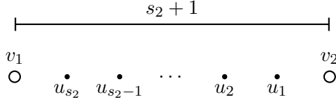
Figure 6.1: The Bethe roots u_k associated to the Yangian invariant |\Psi_{2,1}\rangle of section 4.2.1 arrange into a string between the two inhomogeneities v_1 and v_2 , cf. (6.29) in the complex plane. This string consists of s_2 roots with a uniform real spacing of 1.
