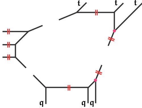
Figure 22: This figure depicts the flopped version of the T_3 geometry and the parallel 5-brane contributions. The circles denote the new topological string vertex introduced by Iqbal and Kozçaz.
