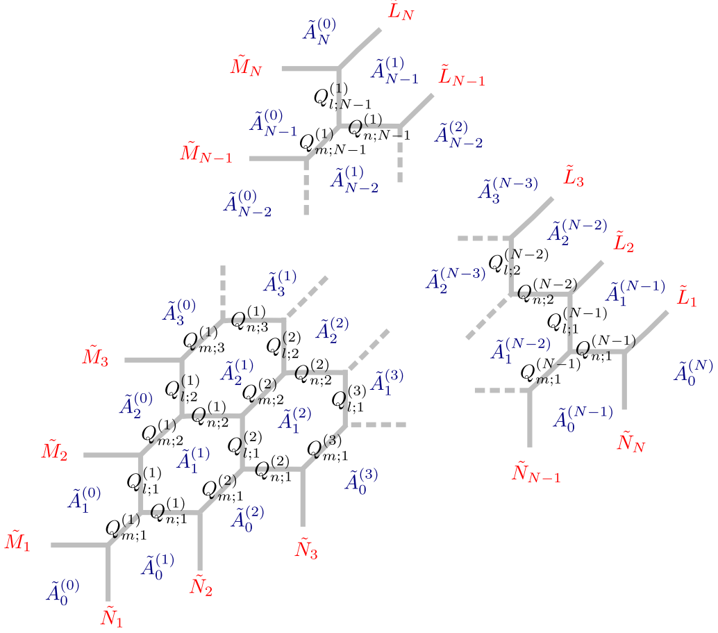
Figure 27: Parametrization for T_N . We denote the Kähler moduli parameters corresponding to the horizontal lines as Q_{n;i}^{(j)} , to the vertical lines as Q_{l;i}^{(j)} , and to tilted lines as Q_{m;i}^{(j)} . We denote the breathing modes as \tilde{A}_i^{(j)} . The index j labels the strips in which the diagram can be decomposed.
