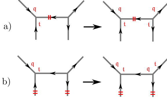
Figure 11: This figure illustrates the way the \mathfrak{t} and \mathfrak{q} variables are placed.
