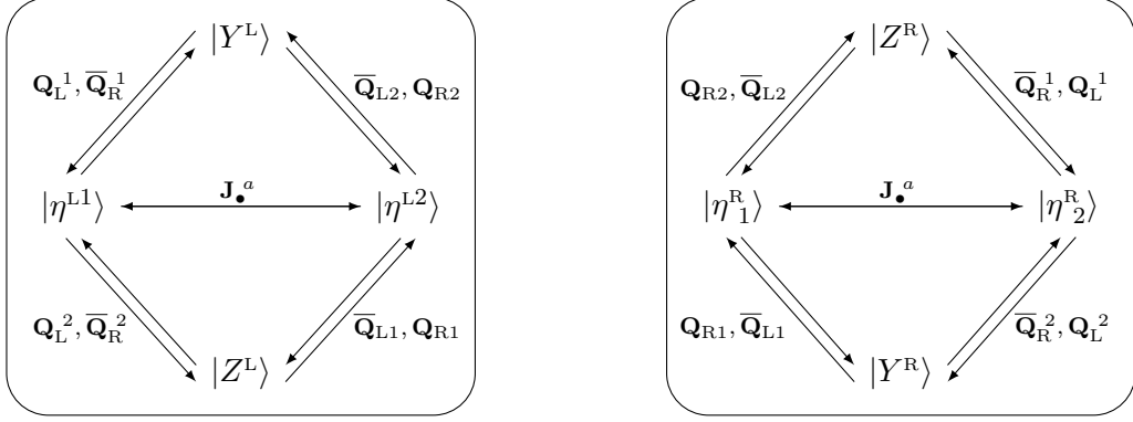
Figure 1: The left and right \mathfrak{psu}(1|1)_{\text{c.e.}}^4 multiplets consists of two bosons Y^{L,R} , Z^{L,R} and of two fermions \eta_{\dot{a}}^{L,R} , corresponding to transverse directions on \text{AdS}_3 \times S^3 . The fermions carry an index \dot{a} of the fundamental representation of \mathfrak{su}(2)_\bullet . Note that off-shell any excitation is charged under all supercharges, whereas on-shell left (respectively right) excitations are charged only under left (respectively right) supercharges. We indicate the supercharges whose action corresponds to the outermost arrows of the diagram. The innermost ones follow by Hermitian conjugation.
