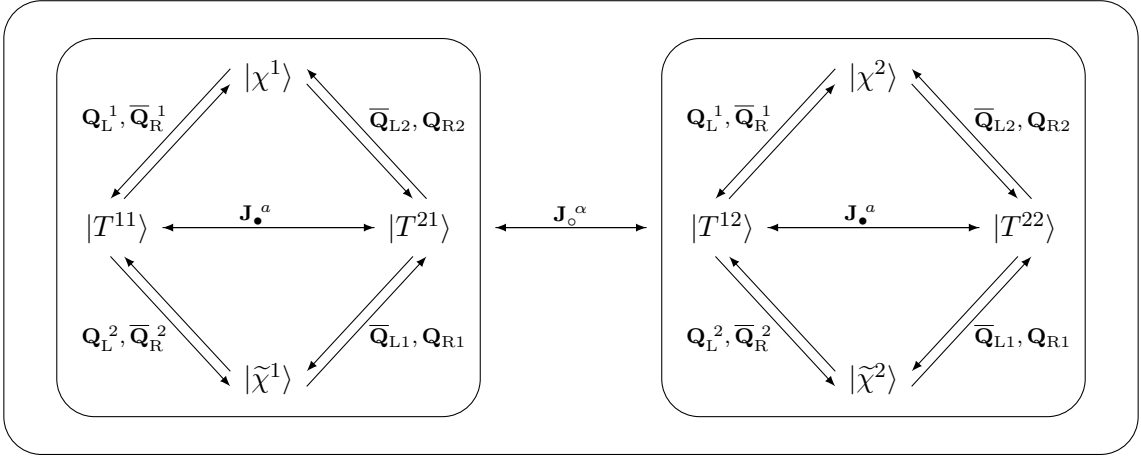
Figure 2: The eight massless excitations form two \mathfrak{psu}(1|1)_{\text{c.e.}}^4 multiplets. The four bosons T^{\hat{a}a} are charged both under \mathfrak{su}(2)_\bullet and \mathfrak{su}(2)_\circ , while the four fermions \chi^a, \tilde{\chi}^a are in the fundamental representation of \mathfrak{su}(2)_\circ only. Again we indicate the charges whose action corresponds to the outermost arrows of the diagram, while the innermost ones follow by Hermitian conjugation. Note how \mathfrak{su}(2)_\circ relates the two \mathfrak{psu}(1|1)_{\text{c.e.}}^4 modules, yielding a single irreducible representation of \mathcal{A} , denoted by a box.
