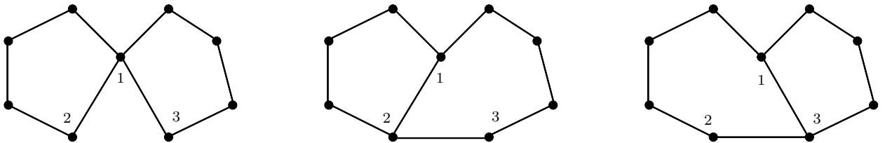
Figure 7: Example of diagrams contributing to G_{n;1} and having a spurious pole at (123) = 0 . This pole cancels in the sum of three diagrams.
