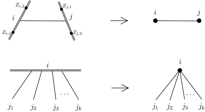
Figure 1: Propagators and vertices in twistor space.
