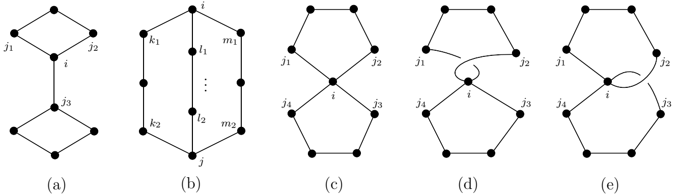
Figure 5: Topologies of twistor diagrams that contribute to G_{n;1} .
