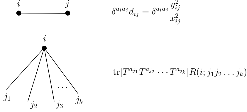
Figure 4: Feynman rules for propagators and vertices in analytic superspace.
