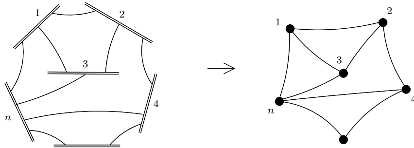
Figure 2: Feynman diagram on twistor space contributing to an n -point correlation function. A double line with label i represents a line in twistor space with moduli (x_i, \theta_i) . Solid lines stand for propagators of twistor superfields and dots denote effective interaction vertices.
