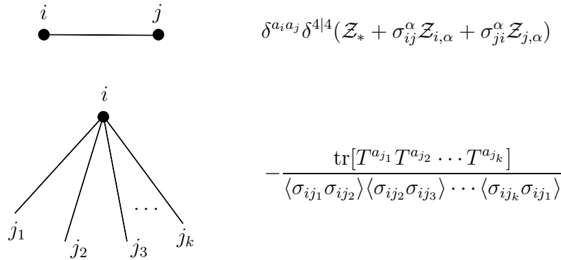
Figure 3: Feynman rules for propagators and vertices in twistor space.
