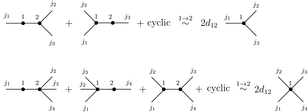
Figure 8: The OPE relations for 3- and 4-point vertices. The expressions on the left-hand side are symmetrised with respect to cyclic shifts of the labels of the external legs.
