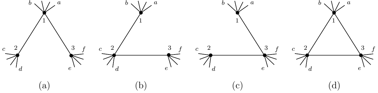
Figure 6: All subgraphs with a potential spurious pole at (123) = 0 . The spurious pole is present in graphs (a), (b) and (c) but cancels in their sum. The graph (d) in fact has no spurious pole at (123) = 0 . In the above diagrams the number of legs coming out of each of the vertices 1,2,3 is arbitrary and we can even have just one leg coming out. For example, we can have a = b or c = d etc. In the graph (d) we can even have no additional legs from the vertices.
