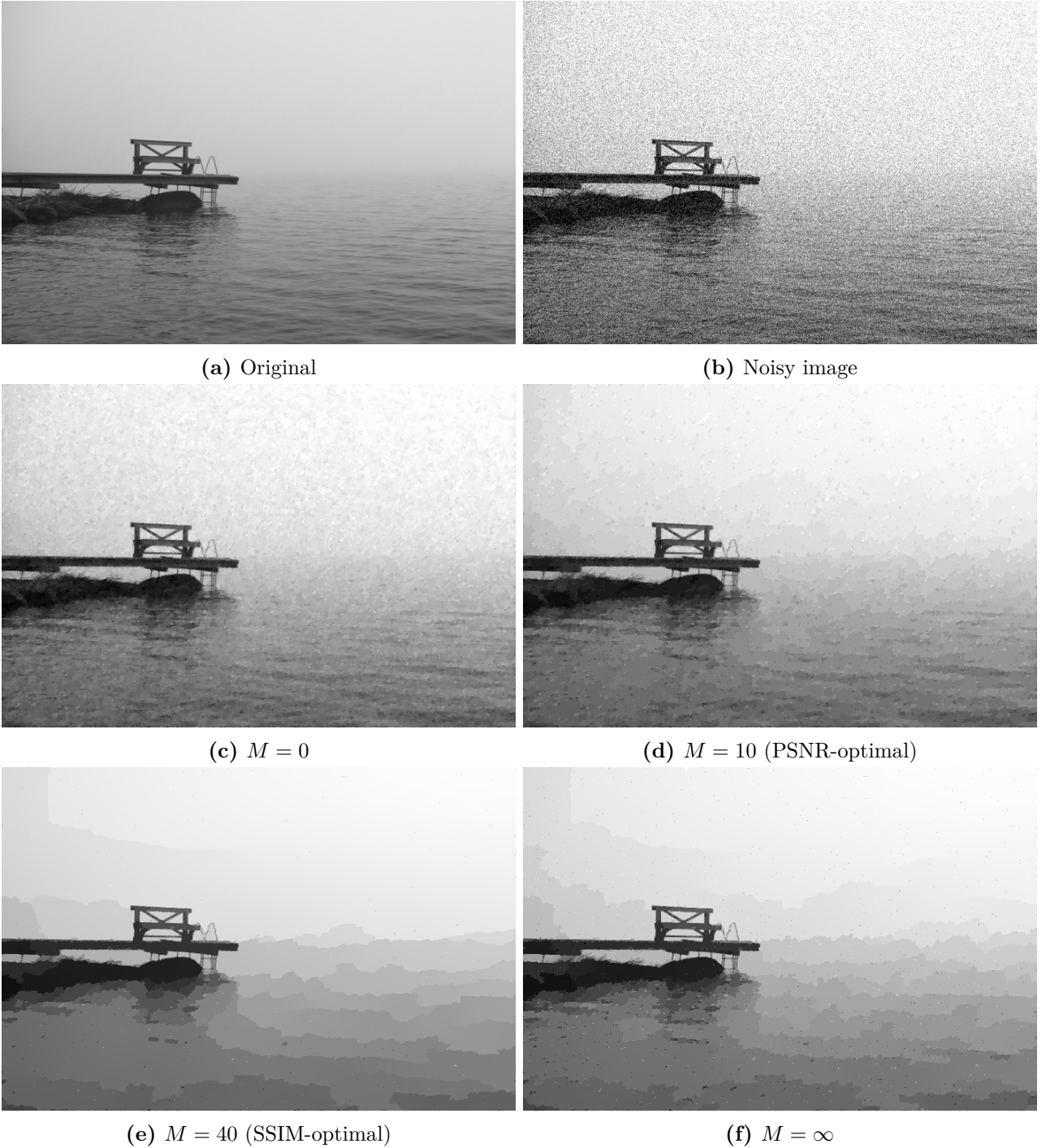
Figure 4: Pier photo: denoising results with noise level \sigma = 30 (Gaussian), for varying cut-off M , fixed q = 0.4 and fixed \alpha^\infty = 0.0207 .
