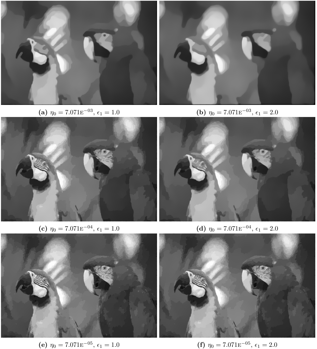
Figure 7: Effect of the \eta term on the parrot photo. Only the first term \eta_1 of the sum is included, with varying convolution width \epsilon_1 and weight \eta_0 . The noise level \sigma = 30 (Gaussian), cut-off M = 10 , exponent q = 0.5 and asymptotic regularisation \alpha^\infty = 0.0253 are fixed.
