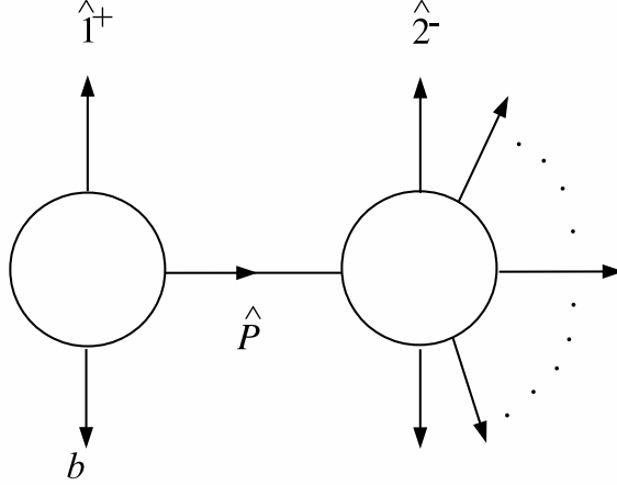
Figure 5: The first BCFW diagram contributing to the double-soft scalar limit.
