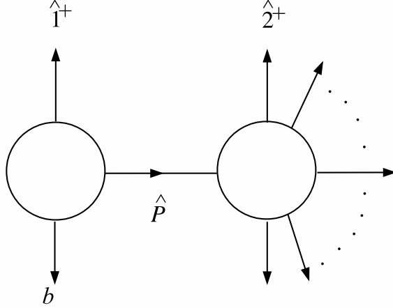
Figure 3: The first class of BCFW diagrams contributing to the double-soft factor for two gravitons. The amplitude on the left-hand side is \overline{\text{MHV}} , and one has to sum over all possible choices of the graviton b .
