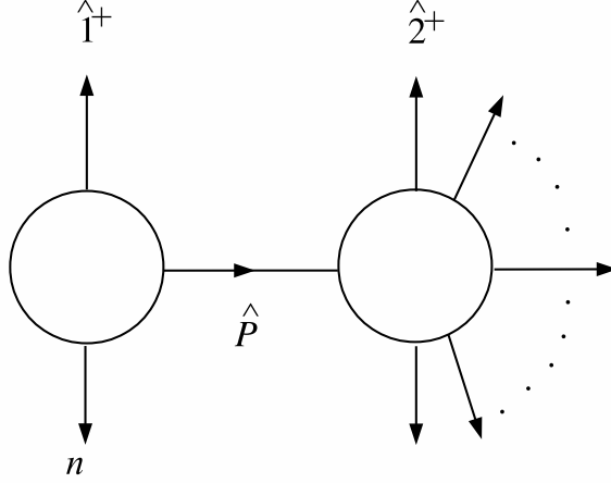
Figure 1: The first BCFW diagram contributing to the double-soft factor. The amplitude on the left-hand side is \overline{\text{MHV}} .
