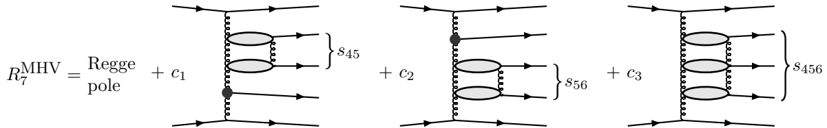
Figure 1: In the seven-point case, the remainder function in every Regge region can be written as a linear combination of the Regge pole contribution, the short cuts in the s_{45} - and s_{56} -channel and the long cut in the combined s_{456} -channel. See [8,9] for details.
