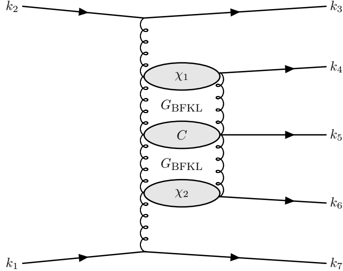
Figure 2: Pictorial representation of eqs. (3.6) and (3.7), with C being the central emission vertex, G_{\text{BFKL}} describing the evolution of the two-Reggeon bound state and \chi_1, \chi_2 being the building blocks of the impact factor.
