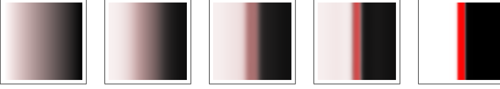
Figure 1: Phase separation process for an initial value which is constant in the vertical direction. The stripe pattern is preserved during the whole evolution. The final state is a local minimizer of the free energy functional F under the constraint of particle number conservation.
