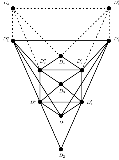
Cases \mathbf{E}_7 and \mathbf{E}_8 .
