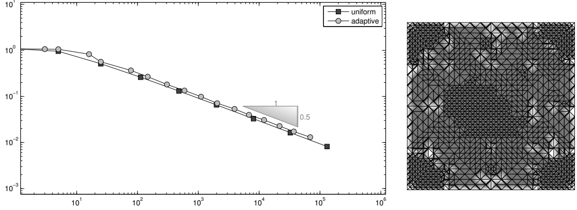
FIGURE 6.9. Convergence history of the energy error as a function of the number of unknowns for uniform and adaptive mesh-refinements (left) and adaptive mesh on level \ell = 9 (right) in Section 6.5
