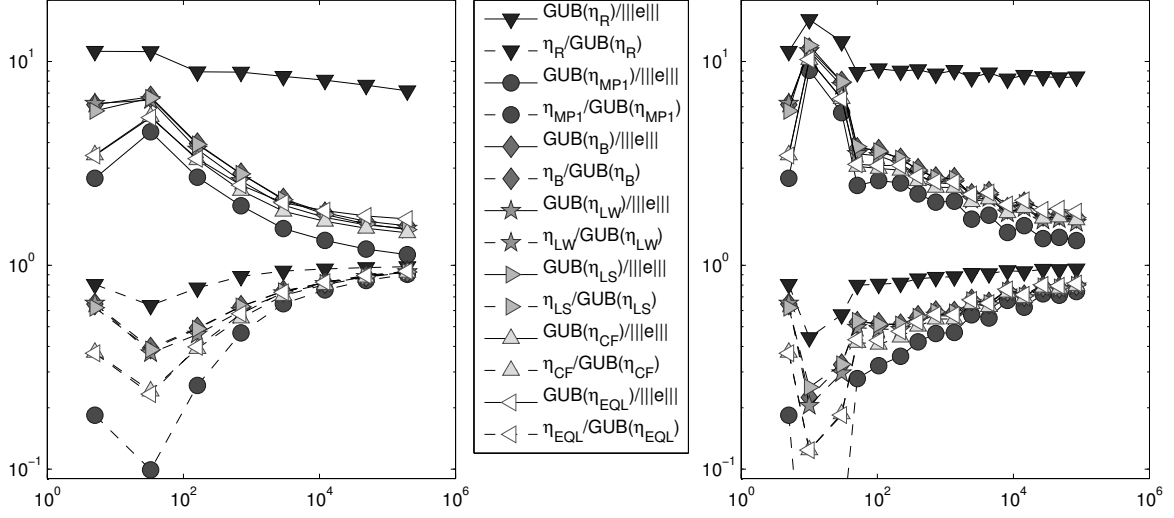
FIGURE 6.4. Efficiency indices of the global upper bound \text{GUB}(\eta_{xyz}) and relative contribution of \eta_{xyz} to the global upper bound as functions of the number of unknowns for uniform (left) and adaptive (right) refinement in Section 6.2.
