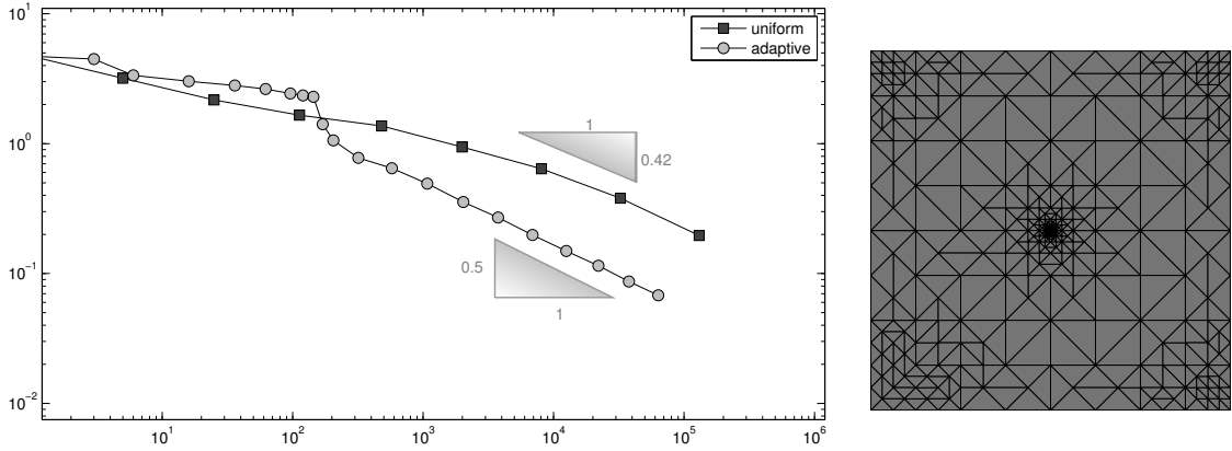
FIGURE 6.5. Convergence history of the energy error as a function of the number of unknowns for uniform and adaptive mesh-refinements (left) and adaptive mesh on level \ell = 12 (right) in Section 6.3
