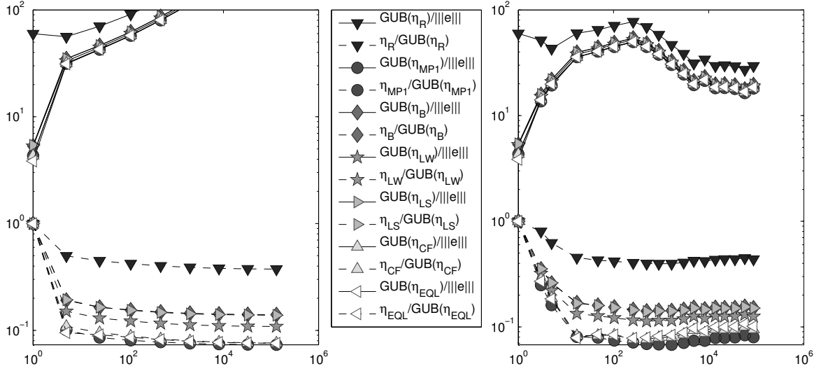
FIGURE 6.8. Efficiency indices of the global upper bound GUB(\eta_{xyz}) and relative contribution of \eta_{xyz} to the global upper bound as functions of the number of unknowns for uniform (left) and adaptive (right) refinement in Section 6.4.
