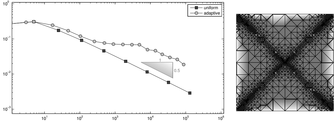
FIGURE 6.7. Convergence history of the energy error as a function of the number of unknowns for uniform and adaptive mesh-refinements (left) and adaptive mesh on level \ell = 9 (right) in Section 6.4
