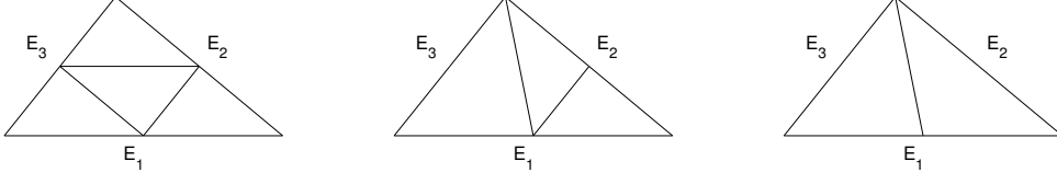
FIGURE 5.1. Red-, blue-, and green-refinement of a triangle.
