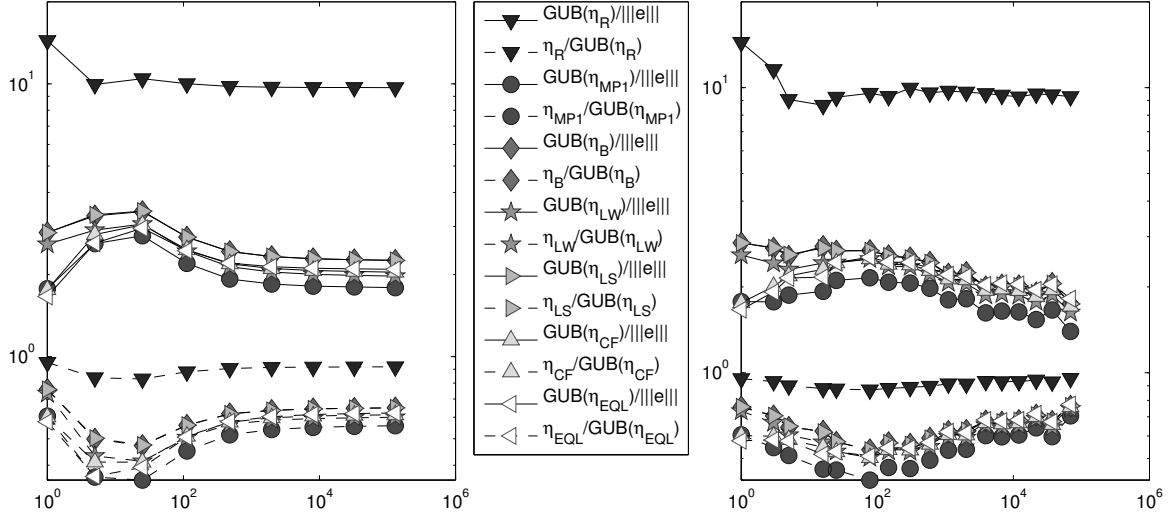
FIGURE 6.10. Efficiency indices of the global upper bound GUB(\eta_{xyz}) and relative contribution of \eta_{xyz} to the global upper bound as functions of the number of unknowns for uniform (left) and adaptive (right) refinement in Section 6.5.
