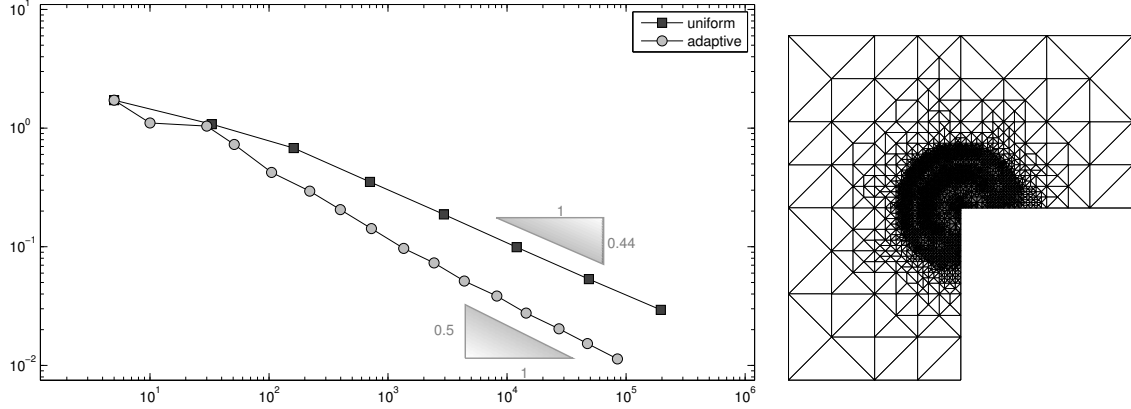
FIGURE 6.3. Convergence history of the energy error as a function of the number of unknowns for uniform and adaptive mesh-refinements (left) and adaptive mesh on level \ell = 9 (right) in Section 6.2
