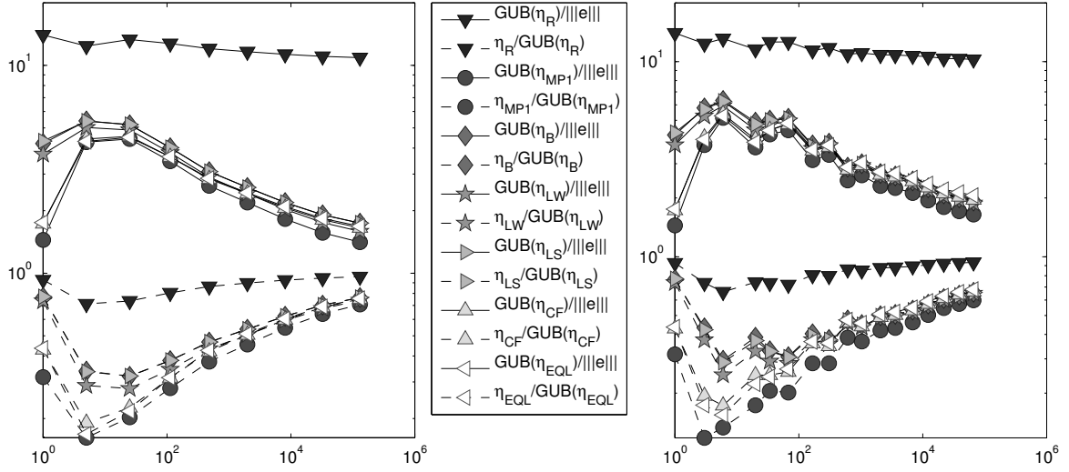
FIGURE 6.2. Efficiency indices of the global upper bound GUB(\eta_{xyz}) and relative contribution of \eta_{xyz} to the global upper bound as functions of the number of unknowns for uniform (left) and adaptive (right) refinement in Section 6.1.
