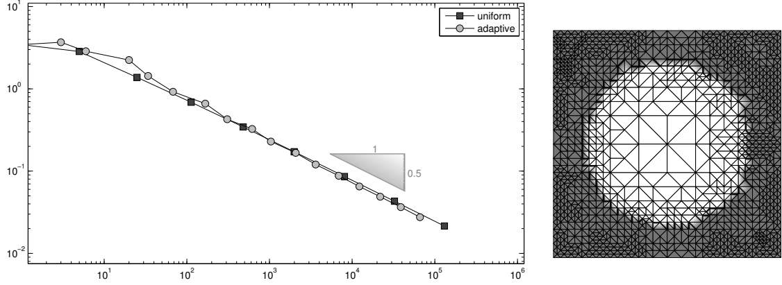
FIGURE 6.1. Convergence history of the energy error as a function of the number of unknowns for uniform and adaptive mesh-refinements (left) and adaptive mesh on level \ell = 9 (right) in Section 6.1
