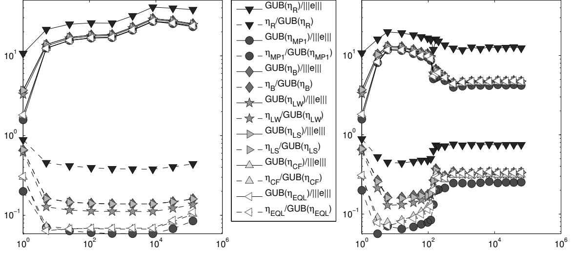
FIGURE 6.6. Efficiency indices of the global upper bound \text{GUB}(\eta_{xyz}) and relative contribution of \eta_{xyz} to the global upper bound as functions of the number of unknowns for uniform (left) and adaptive (right) refinement in Section 6.3.
