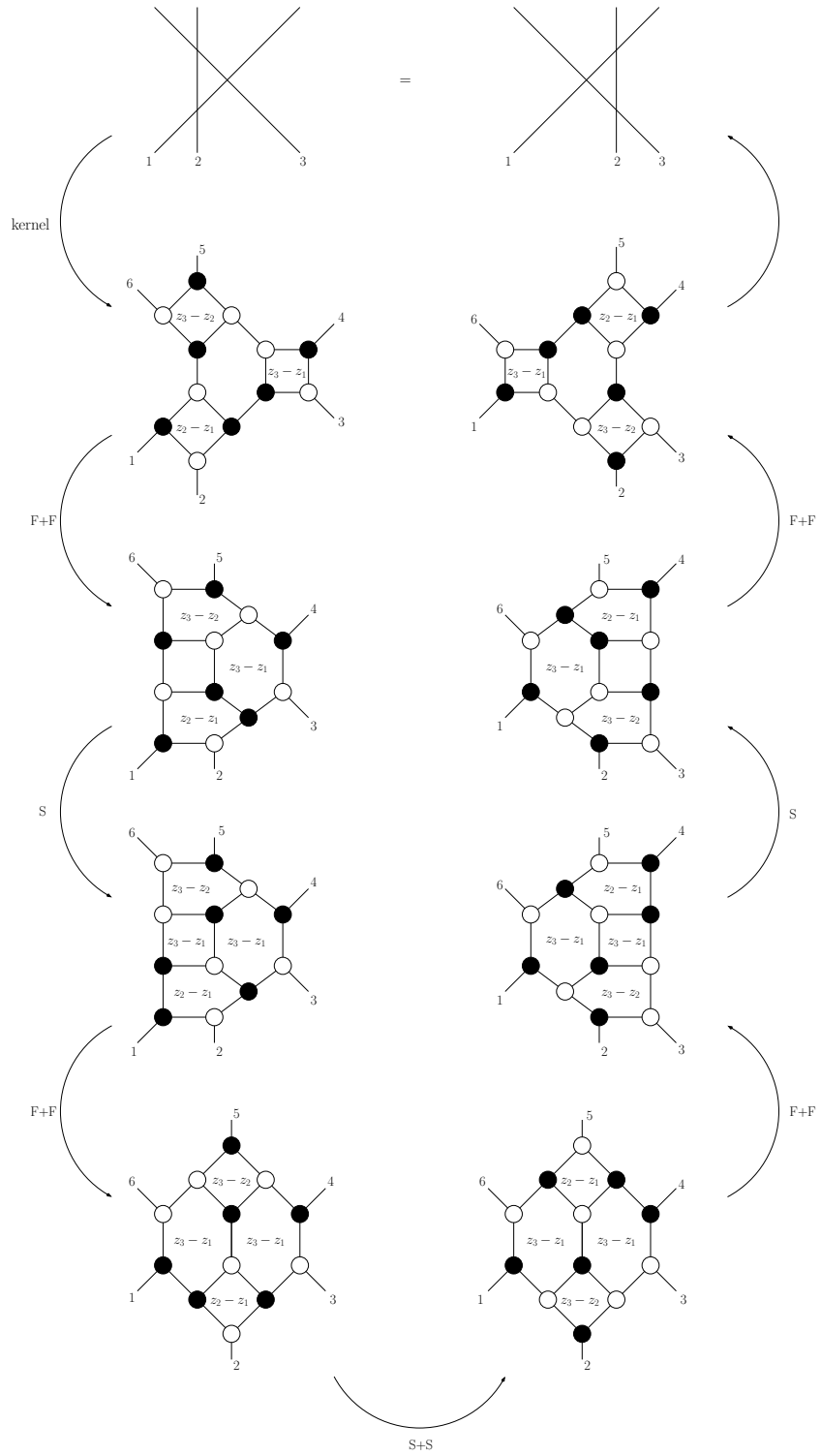
Figure 10: A diagrammatic derivation of the Yang-Baxter equation. At each step we marked whether the square move (S) or flip move (F) was performed.
