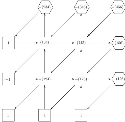
Figure 19: Extended dual graph for the top cell of G(n, k) .
