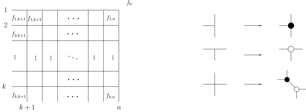
Figure 17: (a) \Gamma -diagram relevant for the top cell of Graßmannian G(n, k) . (b) Dictionary from \Gamma -diagrams to on-shell diagrams.
