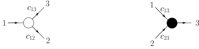
Figure 5: Three-point amplitudes dressed with arrows and weights.
