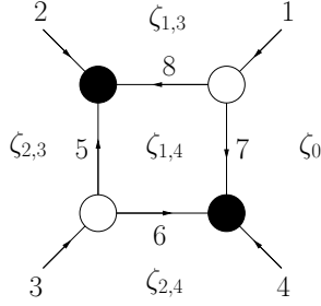
Figure 13: Four-point tree-level.
