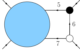
Figure 16: Attaching a single bridge.
