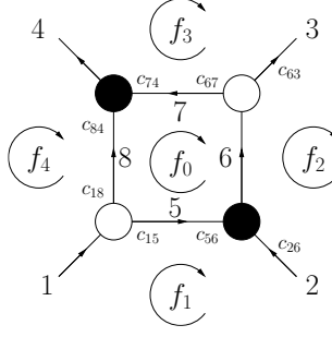
Figure 6: Face variables.
