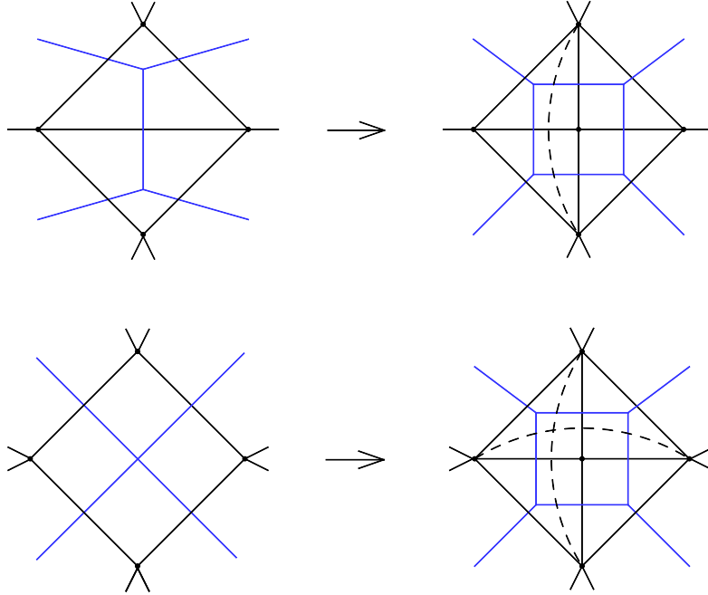
Figure 6: Figures illustrating the rung rule in both position space (black solid lines) and in momentum space (blue lines). In position space, for any square one inserts a vertex with four edges coming from it together with two numerator (dashed) lines. In the first case one of these numerator lines simply cancels the diagonal propagator line. The momentum space graphs give the well-known rung rule for obtaining higher loop amplitude integrands from lower ones.
