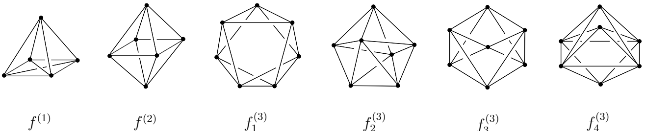
Figure 2: f -graphs up to three loops obtained from the P -graphs in Fig. 1. The one-loop graph f^{(1)} is non-planar, but it becomes planar after multiplying it with the prefactor in (2.20). The two-loop graph f^{(2)} and one of the tree-loop graphs, f_2^{(3)} , are planar. The remaining three-loop graphs f_1^{(3)} , f_3^{(3)} , f_4^{(3)} are non-planar, even including the prefactor in (2.20).
