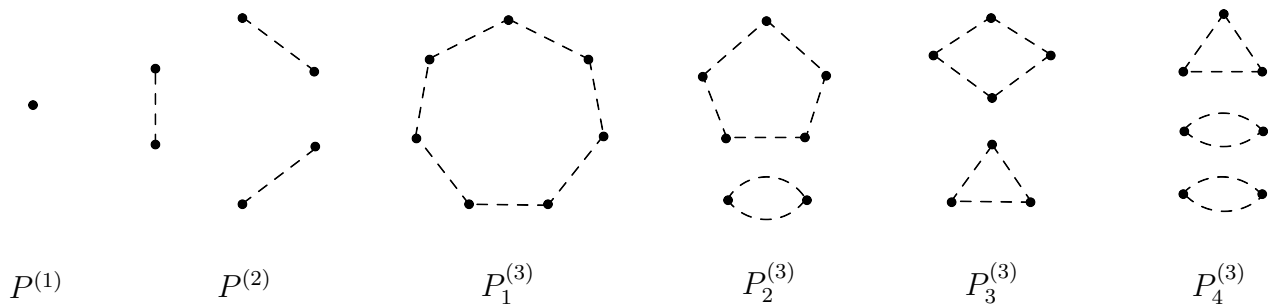
Figure 1: P -graphs up to three loops. The one-loop graph P^{(1)} shrinks to a point corresponding to the constant numerator in (2.25). The two-loop graph P^{(2)} consists of three disconnected segments. At three loops there are four possible graphs, one connected P_1^{(3)} and three disconnected P_2^{(3)} , P_3^{(3)} , P_4^{(3)} .
