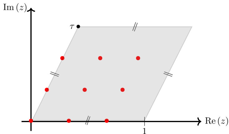
Figure 1: The shaded region represents the elliptic curve \mathbb{C}/(\mathbb{Z} + \mathbb{Z}\tau) , where edges marked by // and \cong are identified. In the setup of teMZVs, points from the lattice \mathbb{Q} + \mathbb{Q}\tau are removed from the elliptic curve. Here we show the example \{0, \frac{1}{3}, \frac{2}{3}\} + \{0, \frac{1}{3}, \frac{2}{3}\}\tau .
