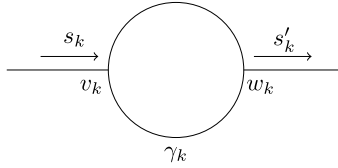
Figure 5: The slopes s_k and s'_k .
