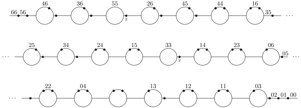
Figure 16: The divisor D' = 2D + \text{div}(\theta) . The function \varphi_{i,j} is assigned to the bridge or loop directly under the label ij , and \varphi_{i,j} + c_{i,j} achieves the minimum uniquely on the labeled region in \Gamma \setminus \text{Supp}(D') .
