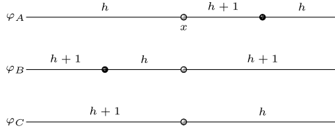
Figure 26: A schematic depiction of the three functions \varphi_A , \varphi_B , \varphi_C from Proposition 11.6, restricted to the subgraph \Gamma_L \subset \Gamma formed by the bridges and the lower half of each loop.
