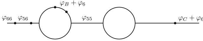
Figure 39: a certificate of independence on \tilde{\Gamma}' .
