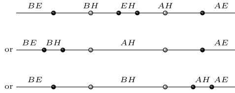
Figure 37: Possibilities for the dependence between \varphi_A, \varphi_B, \varphi_E , and \varphi_H .
