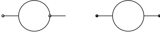
Figure 19: The divisors D (in white) and D_0 (in black) of Example 9.18.
