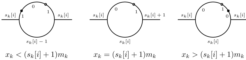
Figure 6: The function (\varphi_i)|_{\gamma_k} when \gamma_k is not lingering.
