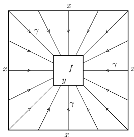
FIGURE 30. The isomorphism \pi_n(X, y) \rightarrow \pi_n(X, x) determined by a path x \rightsquigarrow y .
