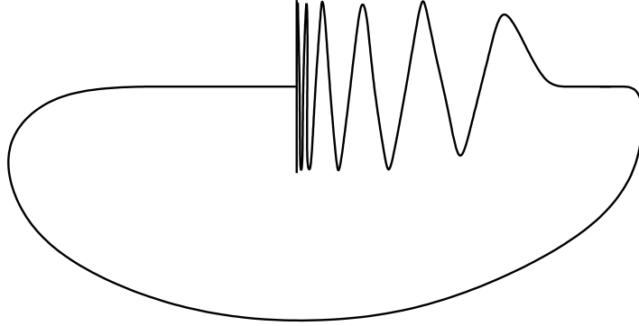
FIGURE 33. The Warsaw circle: a space that is weakly contractible but not contractible.
