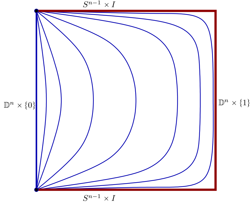
FIGURE 34. Foliating the interior of \mathbb{D}^n \times I by a 1-parameter family of n -disks with identical boundary at S^{n-1} \times \{0\} .
