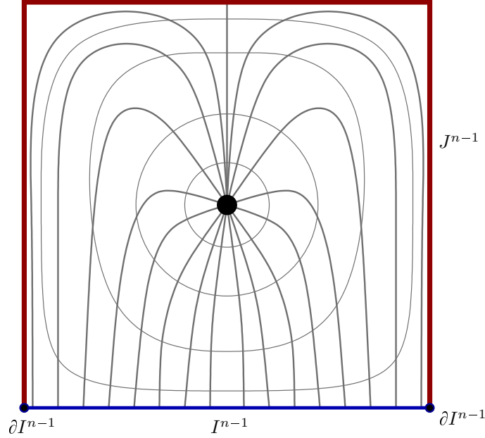
FIGURE 32. A homeomorphism of pointed pairs (I^n/J^{n-1}, I^{n-1}/\partial I^{n-1}) \cong (\mathbb{D}^n, S^{n-1}) .
