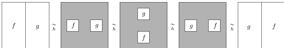
FIGURE 31. A homotopy to demonstrate the reason why \pi_2(X) is abelian. A similar trick works for \pi_n(X) with any n \geq 2 , but not for n = 1 .
