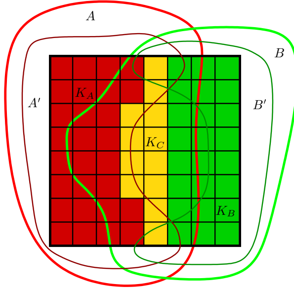
FIGURE 36. The subcomplexes K_C = K_A \cap K_B \subset K_A, K_B \subset I^k in the proof of Lemma 68.11.
