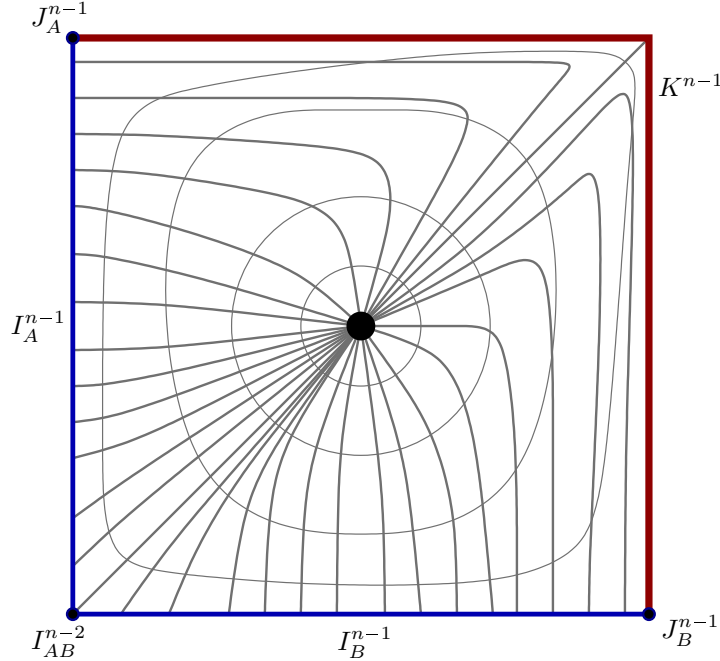
FIGURE 37. A homeomorphism I^n/K^{n-1} \cong \mathbb{D}^n identifying I_A^{n-1}/J_A^{n-2} and I_B^{n-1}/J_B^{n-2} with the hemispheres \mathbb{D}_+^{n-1} and \mathbb{D}_-^{n-1} respectively in the boundary of \mathbb{D}^n , meeting along the equator I_{AB}^{n-2}/\partial I_{AB}^{n-2} \cong S^{n-2} = \mathbb{D}_+^{n-1} \cap \mathbb{D}_-^{n-1} .
