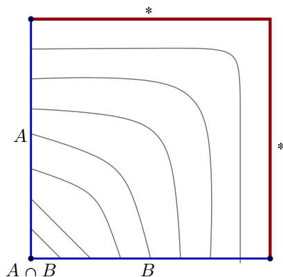
FIGURE 38. Reinterpreting maps I^2 \rightarrow X that satisfy the conditions of (70.1) as paths in the path space P(A, B) from A \cap B to the base point.
